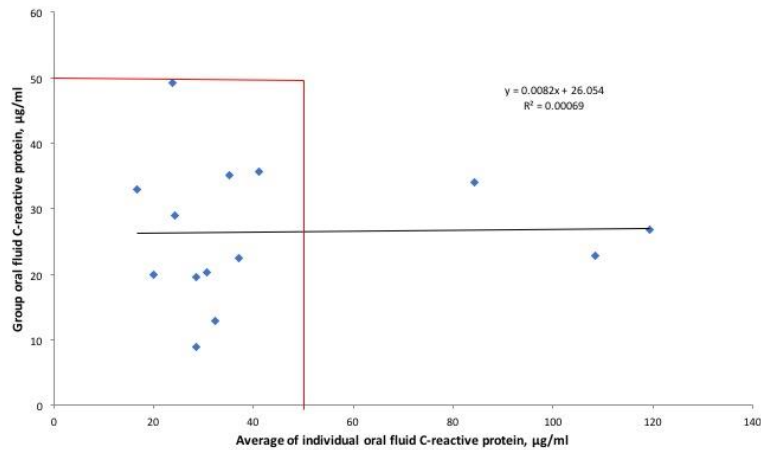
Figure 3. Correlation between oral fluid C-reactive protein concentration determined by the average of individual oral fluid sampling and one-point group sampling using cotton rope ( r=0.026 , P=0.929 ). The C-reactive protein concentrations within the red-rectangle represent healthy pigs, while C-reactive protein concentrations outside of the red-rectangle represent unhealthy pigs.
