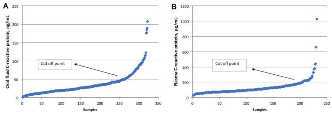
Figure 1. Cut-off points to discriminate healthy and unhealthy pigs for C-reactive protein concentrations in oral fluid (A) and plasma (B) samples.
